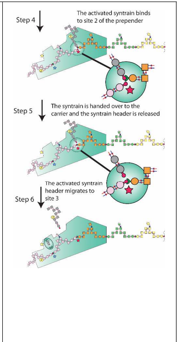
Figure 22. Intermediate steps for syntrain assembly.
