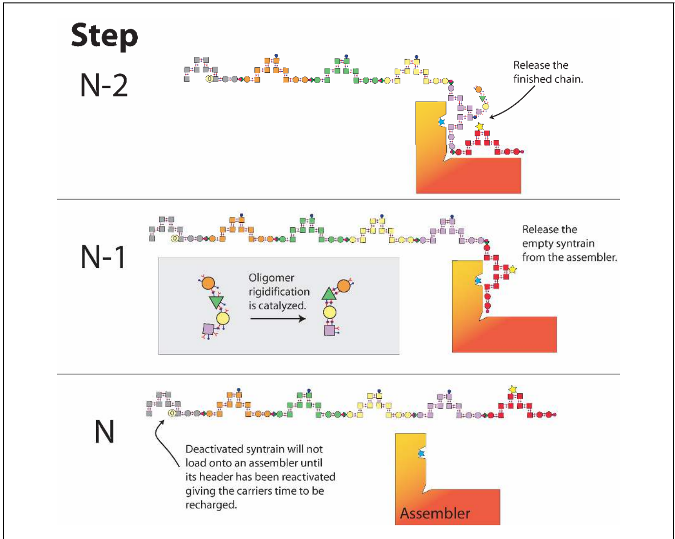
Figure 17. The final steps of oligomers synthesis are shown.
